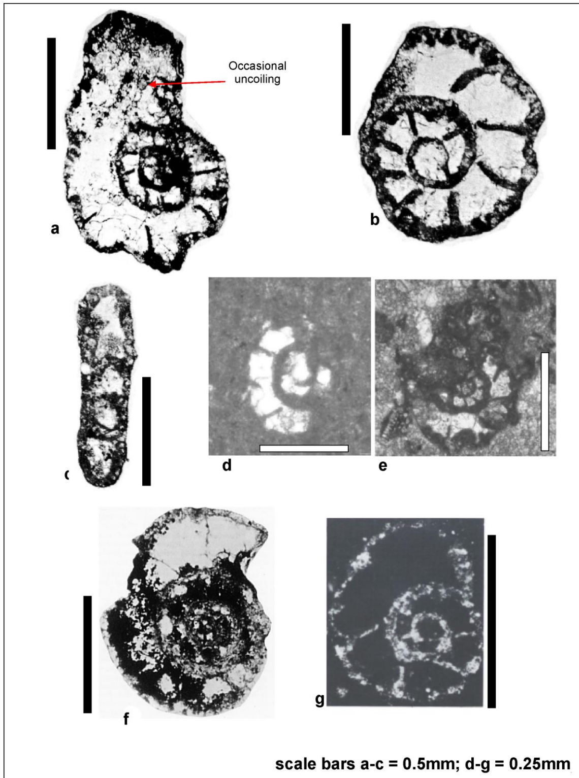
Fig. 4 a – Hemicyclammina whitei (Henson). Specimen labelled as “ Hemicyclammina , nov. sp.?” by Hamaoui (1965) (subsequently H. evoluta sensu Hamaoui 1979) IT.649 – 19718 – 63.5/196. Type Hazera Formation, Israel. Note uncoiling. b – Hemicyclammina whitei (Henson). Specimen labelled as “ Hemicyclammina , nov. sp.?” by Hamaoui (1965) (subsequently H. evoluta sensu Hamaoui 1979) IT.686 – 19696 – 63.5/156. Type Hazera Formation, Israel. c – Hemicyclammina whitei (Henson). Specimen labelled as “ Hemicyclammina , nov. sp.?” by Hamaoui (1965) (subsequently H. evoluta sensu Hamaoui 1979) IT.687 – 19699 – 63.5/161. Type Hazera Formation, Israel. d – Hemicyclammina ? sp. Specimen labelled as “ Hemicyclammina sigali ” by Hosseini et al. (2016) Sample ARP 976. Lar outcrop, Iranian Zagros. e – Hemicyclammina ? sp. Specimen labelled as “ Hemicyclammina sigali ” by Hosseini et al. (2016) Sample ARP 261. Anneh outcrop, Iranian Zagros. f – ? Hemicyclammina whitei (Henson). Specimen labelled as Ismailia neumannae n. gen., n. sp. by El-Dakkak (1974) from Djebel Nezzazat, Sinai, Egypt. g – ? Hemicyclammina whitei (Henson). Specimen labelled as Sinainella aegyptiaca n. gen., n. sp. by El-Dakkak (1975) from Djebel Nezzazat, Sinai, Egypt.
