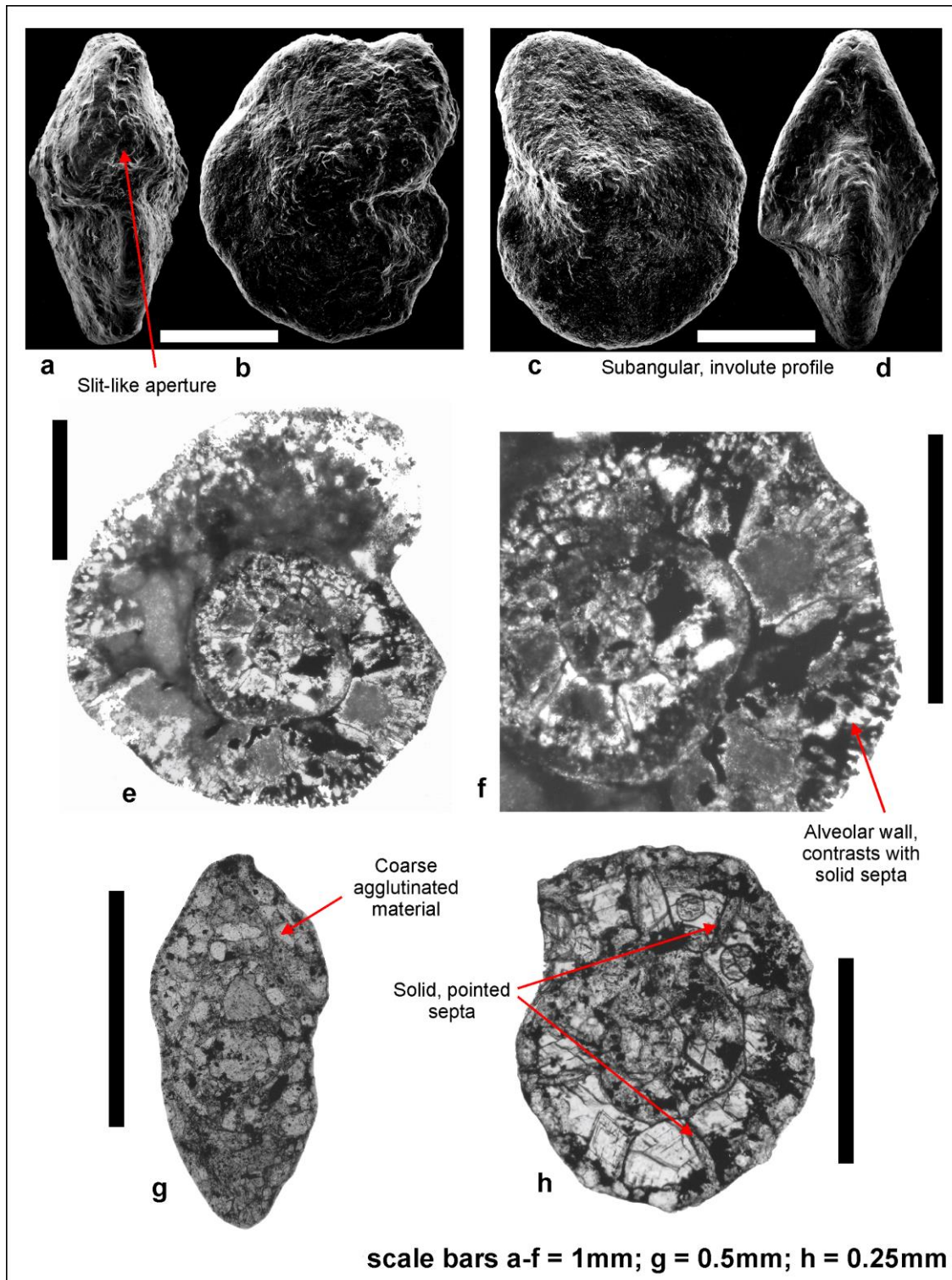
Fig. 1 a, b – Holotype of Hemicyclammina whitei (Henson). Natural History Museum, London Specimen IPC M/3723; NHMUK PM P35798. Dukhan-3 well, Qatar, 3542-3543' reinterpreted as latest Albian (see text). Image reproduced courtesy of the Trustees of the Natural History Museum. c, d – Paratype of Hemicyclammina whitei (Henson). Natural History Museum, London Specimen IPC M/3724; NHMUK PM P35799. Dukhan-3 well, Qatar, 3542-3543' reinterpreted as latest Albian (see text). Image reproduced courtesy of the Trustees of the Natural History Museum. e, f – Paratype of Hemicyclammina whitei (Henson). Natural History Museum, London Specimen IPC M/3722; NHMUK PM P35797. Dukhan-3 well, Qatar, 3542-3543' reinterpreted as latest Albian (see text). Probable microspheric form. Note alveolar ( sensu Hottinger, 2006) wall and solid short septa. Image reproduced courtesy of the Trustees of the Natural History Museum. g – Hemicyclammina whitei (Henson). Natural History Museum, London Specimen IPC M/8357. Rumaila-1 well, Iraq, 8010-8415' Nahr Umr Formation, Albian. Probable macrospheric form. Image reproduced courtesy of the Trustees of the Natural History Museum. h – Hemicyclammina whitei (Henson). Natural History Museum, London Specimen IPC M/8378. Rumaila-1 well, Iraq, 8010-8415' Nahr Umr Formation, Albian. Short, pointed septa clearly visible. Image reproduced courtesy of the Trustees of the Natural History Museum.
