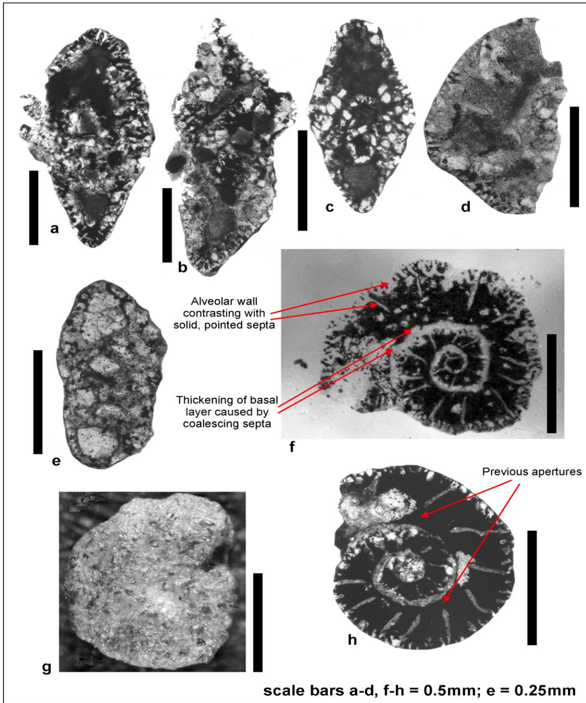
Fig. 2 a - Paratype of Hemicyclammina whitei (Henson). Natural History Museum, London Specimen IPC M/3725; NHMUK PM P35800. Dukhan-3 well, Qatar, 3542-3543' reinterpreted as latest Albian (see text). Alveolar ( sensu Hottinger, 2006) wall clearly visible. Image reproduced courtesy of the Trustees of the Natural History Museum. b - Paratype of Hemicyclammina whitei (Henson). Natural History Museum, London Specimen IPC M/3744. Dukhan-3 well, Qatar, 3542-3543' reinterpreted as latest Albian (see text). Image reproduced courtesy of the Trustees of the Natural History Museum. c - Paratype of Hemicyclammina whitei (Henson). Natural History Museum, London Specimen IPC M/3743. Dukhan-3 well, Qatar, 3542-3543' reinterpreted as latest Albian (see text). Image reproduced courtesy of the Trustees of the Natural History Museum. d - Paratype of Hemicyclammina whitei (Henson). Natural History Museum, London Specimen IPC M/3745. Dukhan-3 well, Qatar, 3542-3543' reinterpreted as latest Albian (see text). Note alveolar ( sensu Hottinger, 2006) wall and solid short septa. Image reproduced courtesy of the Trustees of the Natural History Museum. e - Hemicyclammina whitei (Henson). Natural History Museum, London Specimen IPC M/8378. Rumaila-1 well, Iraq, 8010-8415' Nahr Umr Formation, Albian. Image reproduced courtesy of the Trustees of the Natural History Museum. f - Hemicyclammina whitei (Henson). Paratype of Hemicyclammina sigali Maync. United States Natural History Museum Specimen PAL 324620. Middle Cenomanian, near Morsott, Algeria. g - Hemicyclammina whitei (Henson). Holotype of Hemicyclammina sigali Maync. United States Natural History Museum Specimen PAL 370417. Middle Cenomanian, near Morsott, Algeria. h - Hemicyclammina whitei (Henson). Specimen labelled as " Hemicyclammina sigali Maync". Natural History Museum, London Specimen IPC M/8372. Rumaila-1 well, Iraq, 9008' Nahr Umr Formation, Albian. Image reproduced courtesy of the Trustees of the Natural History Museum
